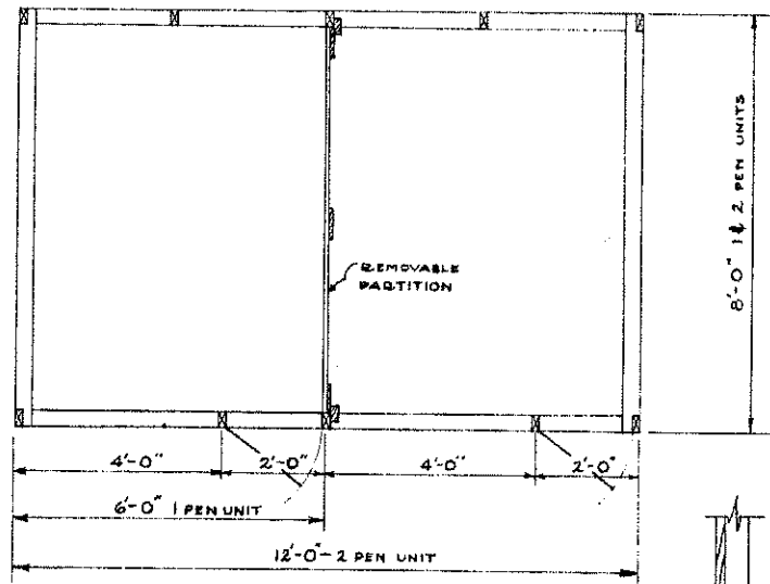
PLAN SCALE \frac{1}{2} " = 1'-0"
