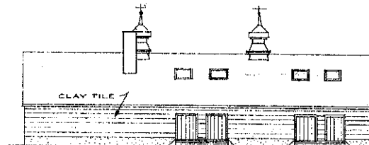
WEST ELEVATION SCALE \frac{1}{8}'' = 1'-0''
