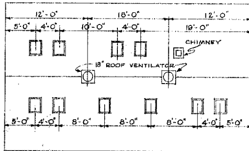
ROOF PLAN SCALE \frac{1}{8}'' = 1'-0''
