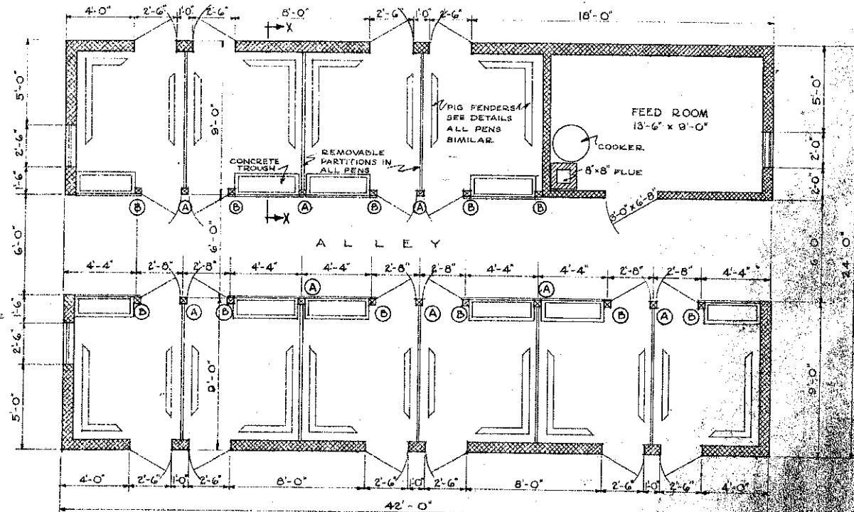
FLOOR PLAN SCALE \frac{1}{4}'' = 1'-0''
