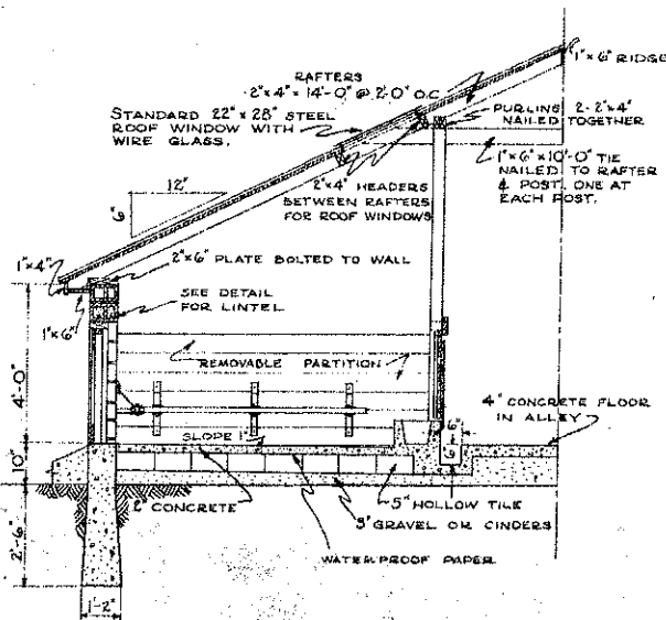
HALF CROSS SECTION SCALE \frac{1}{8}'' = 1'-0''
