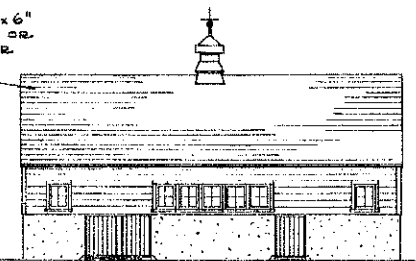
EAST ELEVATION SCALE \frac{1}{8}'' = 1'-0''
