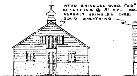
END ELEVATION SCALE \frac{1}{8}'' = 1'-0''
