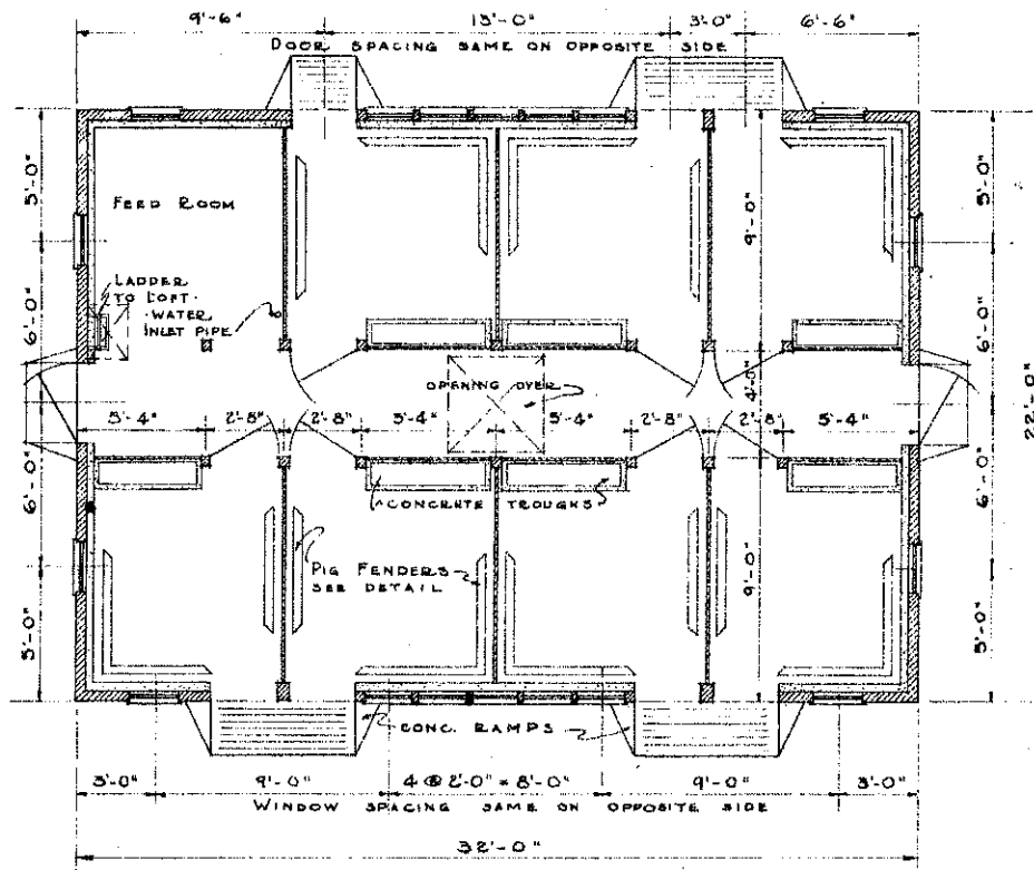
FLOOR PLAN SCALE \frac{1}{4}'' = 1'-0''
