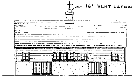
WEST ELEVATION SCALE \frac{1}{8}'' = 1'-0''
