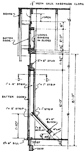
SECTION B-B SHOWING FRAMING SCALE \frac{1}{2} " = 1'-0"
