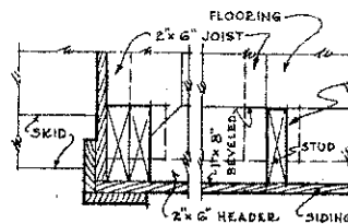
PLAN AT E-E (SEE END ELEVATION) SCALE \frac{1}{2} " = 1'-0"
