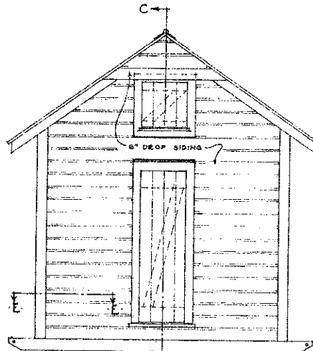
SIDE ELEVATION SCALE \frac{1}{2} " = 1'-0"
