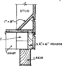
SECTION F-F (SEE FLOOR PLAN) SCALE \frac{1}{2} " = 1'-0"
