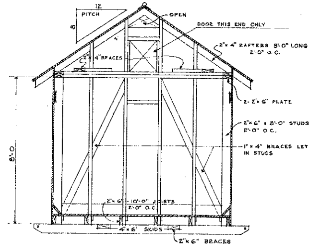
SECTION A-A SHOWING FRAMING SCALE \frac{1}{2} " = 1'-0"
