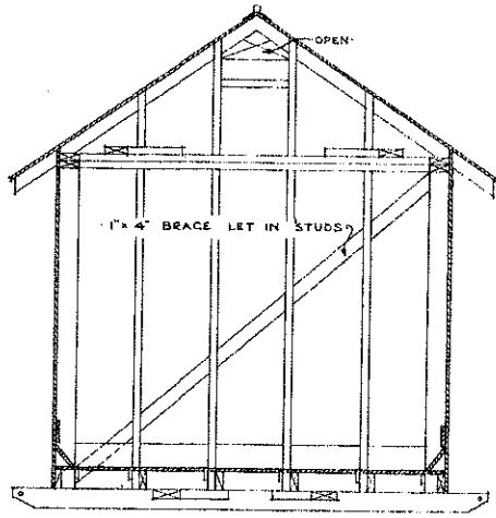
SECTION B-B SHOWING FRAMING SCALE \frac{1}{2} " = 1'-0"
