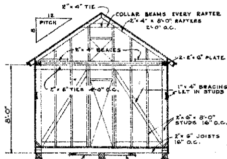
SECTION A-A SHOWING FRAMING SCALE \frac{1}{4} " = 1'-0"
