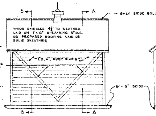
SIDE ELEVATION SCALE \frac{1}{4} " = 1'-0"
