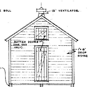
END ELEVATION SCALE \frac{1}{4} " = 1'-0"
