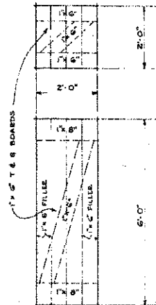
ELEVATION OF BATTEN DOORS SCALE \frac{1}{4} " = 1'-0"
