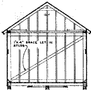
SECTION B-B SHOWING FRAMING SCALE \frac{1}{4} " = 1'-0"
