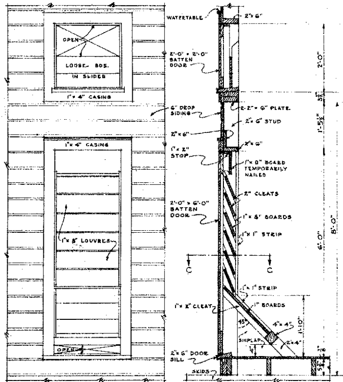
ELEVATION (WITH BATTEN DOORS NOT SHOWN)
