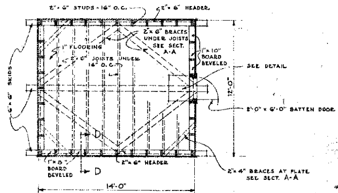
FLOOR PLAN SCALE \frac{1}{4} " = 1'-0"
