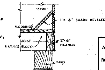
SECTION D-D (SEE PLAN ABOVE) SCALE \frac{1}{4} " = 1'-0"
