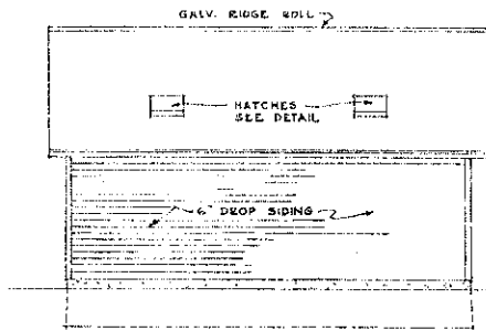
EAST ELEVATION
