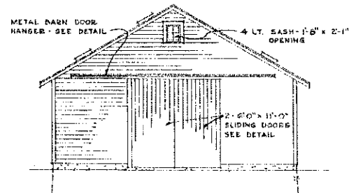
NORTH AND SOUTH ELEVATION
