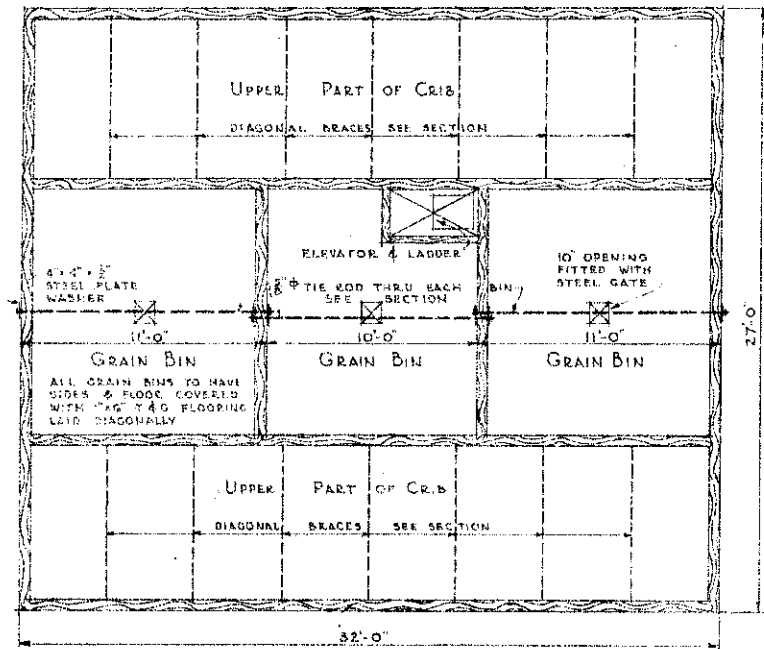
BIN FLOOR PLAN SCALE \frac{1}{2} " = 1'-0"
