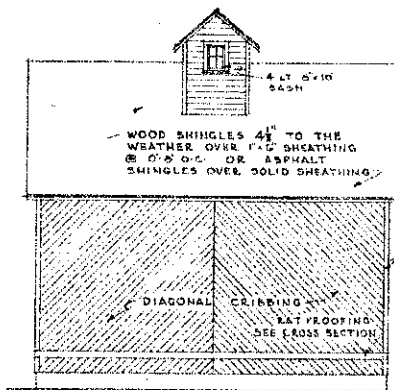
SIDE ELEVATION SCALE \frac{1}{2} " = 1'-0"
