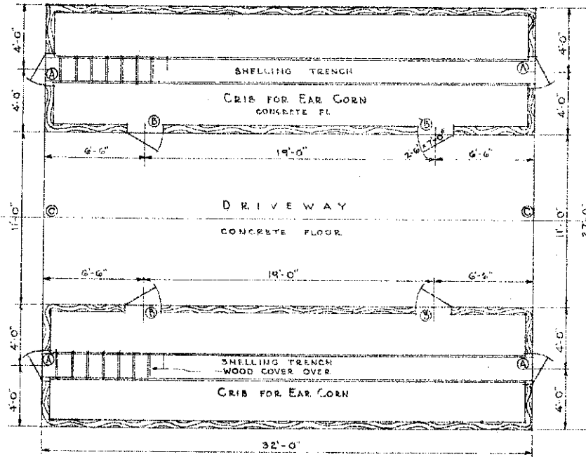
GROUND FLOOR PLAN SCALE \frac{1}{2} " = 1'-0"
