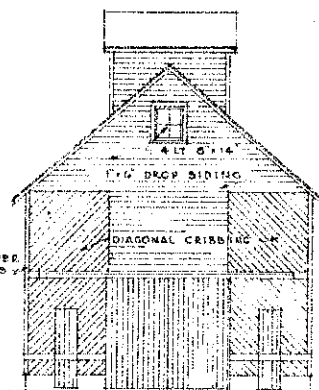
END ELEVATION SCALE \frac{1}{2} " = 1'-0"
