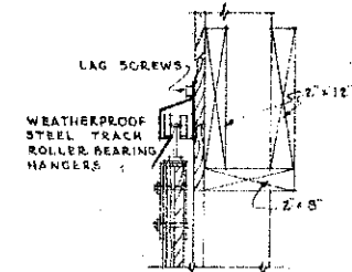
DETAIL OF LINTEL OVER DRIVEWAY DOOR SCALE \frac{1}{2} " = 1'-0"
