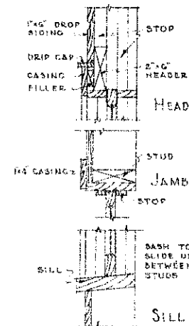
TYPICAL WINDOW DETAILS SCALE \frac{1}{2} " = 1'-0"
