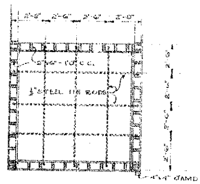
PLAN OF TIE RODS IN CONCRETE BIN FLOORS SCALE 1/4" = 1'-0"
