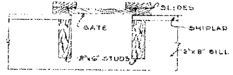
DETAIL OF CHUTE OPENING SCALE 1/2" = 1'-0"
