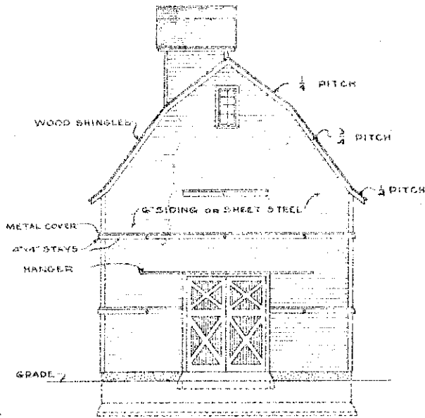
FRONT ELEVATION 1/2" = 1'-0"
