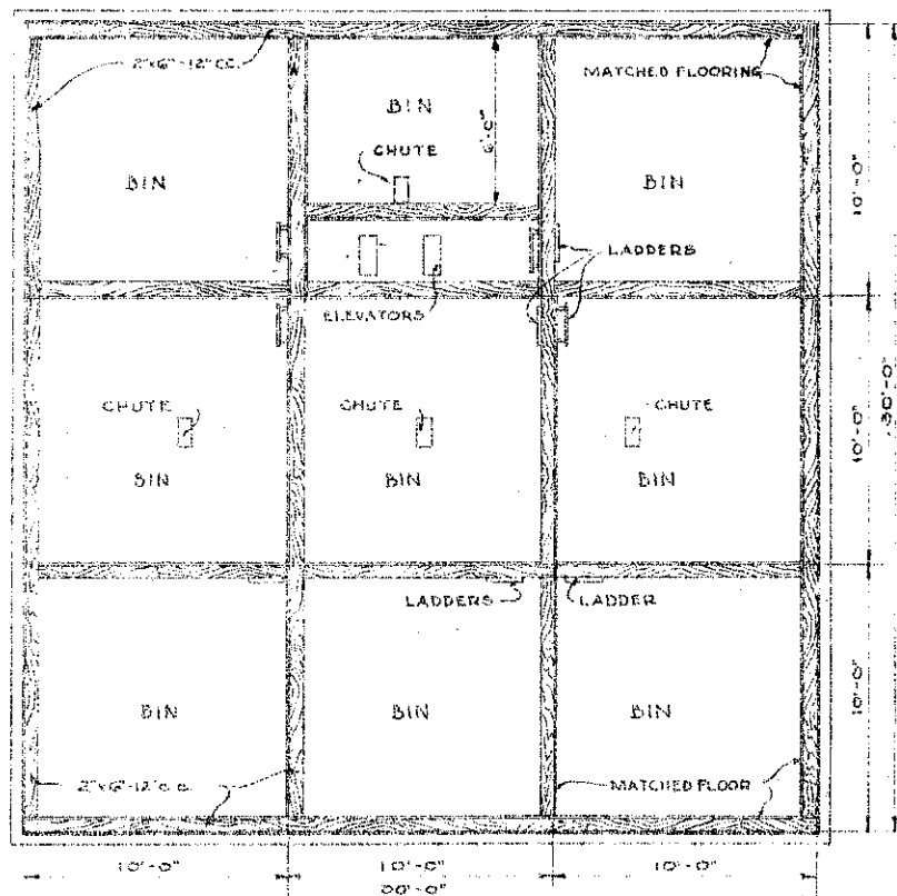
PLAN ABOVE DRIVEWAY
