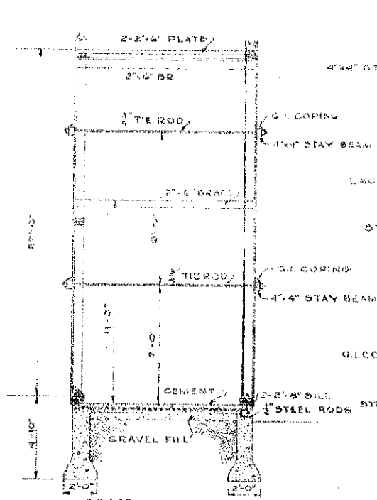
SECTION OF BINS SCALE 1/4" = 1'-0"
