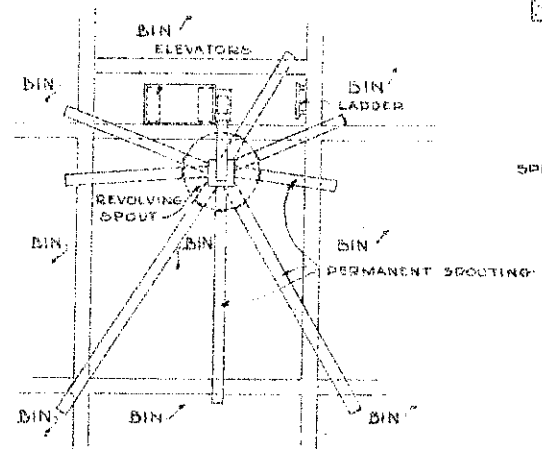
PLAN OF SPOUTING AT ELEVATOR HEAD SCALE 1/4" = 1'-0"
