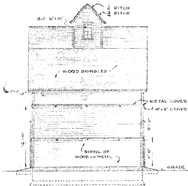
SIDE ELEVATION 1/2" = 1'-0"
