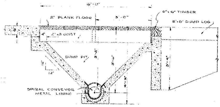
DUMP PIT DETAIL SCALE 3/8" = 1'-0"
