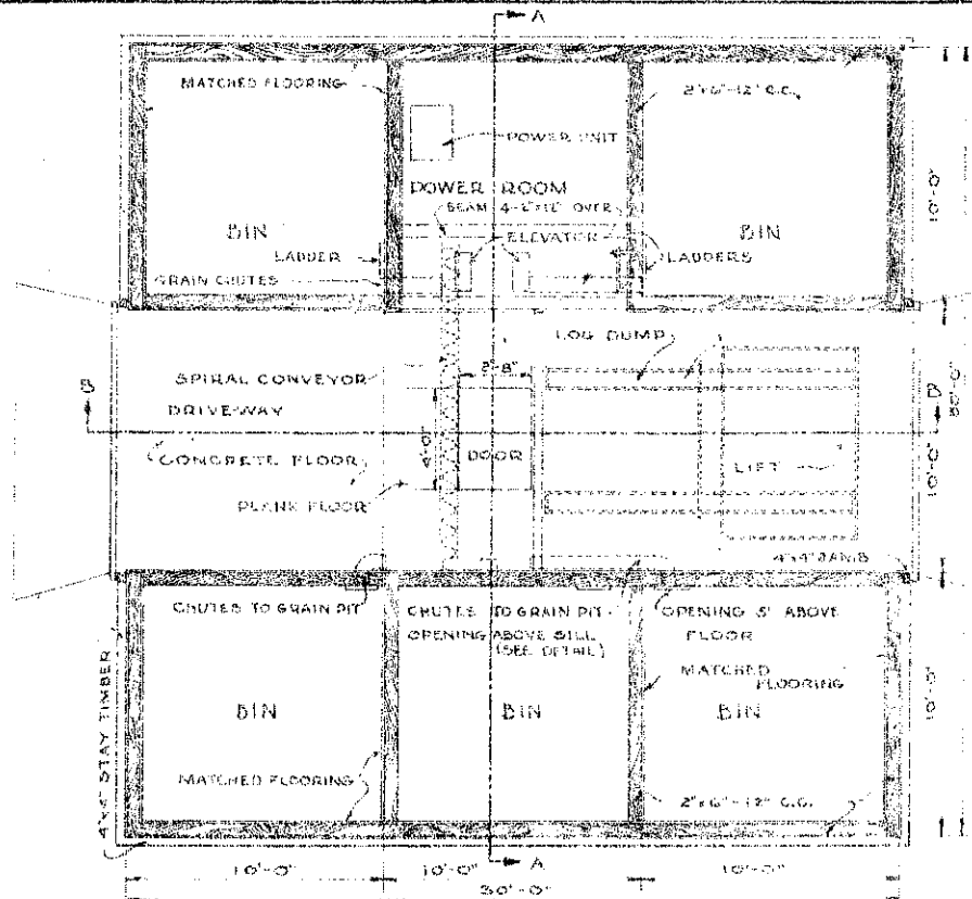
PLAN AT DRIVEWAY
