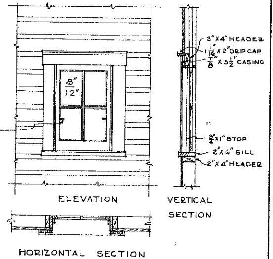
DETAILS OF WINDOWS SCALE \frac{3}{4} " = 1'-0"
