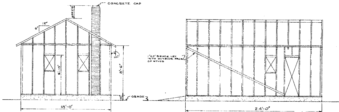
REAR WALL FRAMING SCALE \frac{1}{4}'' = 1'-0''
