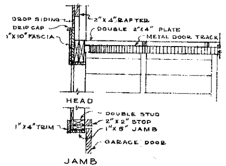
DETAILS OF GARAGE DOOR OPENING SCALE \frac{3}{4} " = 1'-0"
