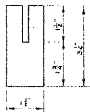
DETAIL SCALE 6" = 1'-0"
