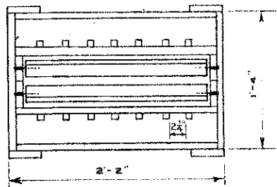
TOP VIEW SCALE 1\frac{1}{2}'' = 1'-0''
