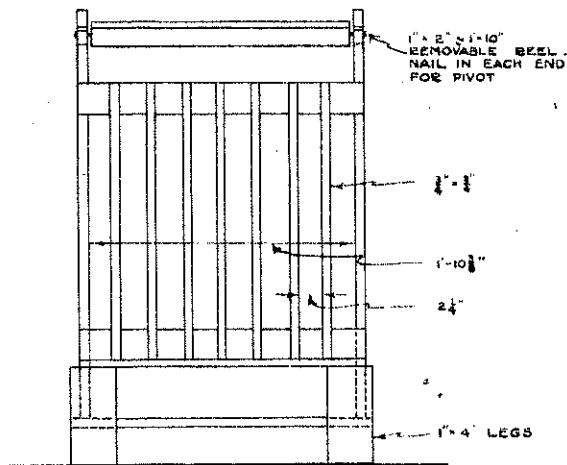
FRONT VIEW SCALE 1\frac{1}{2}'' = 1'-0''
