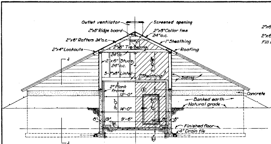
SECTION H-H
