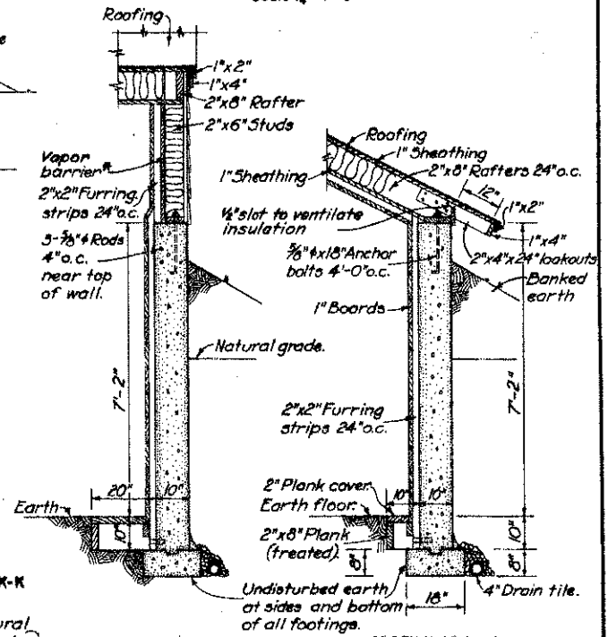
SECTION AT J-J SECTION AT K-K TYPICAL WALL SECTIONS Scale 1/2" = 1'-0"
