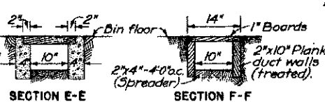
DUCT DETAILS Scale \frac{3}{4}'' = 1'-0''
