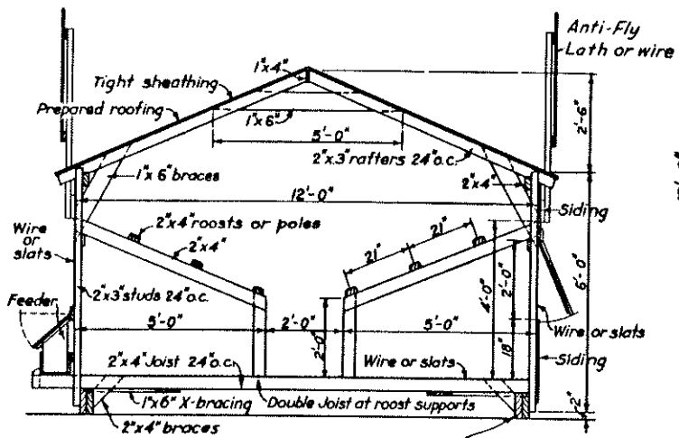
CROSS SECTION
