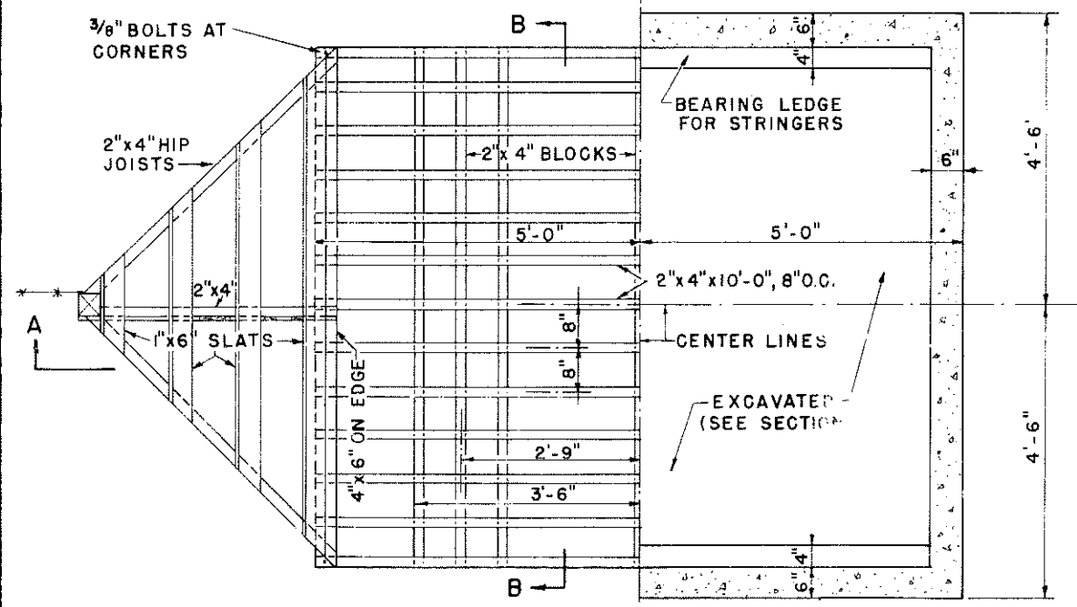
1/2 OF PLAN
