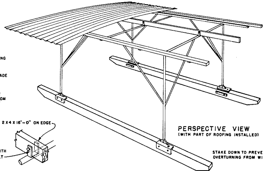
RIDGE DETAIL
