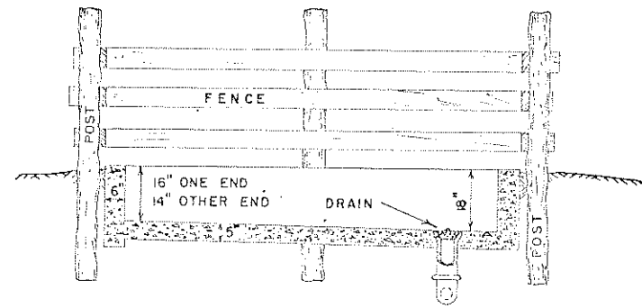
CROSS SECTION 0 1 2 3 FT.
