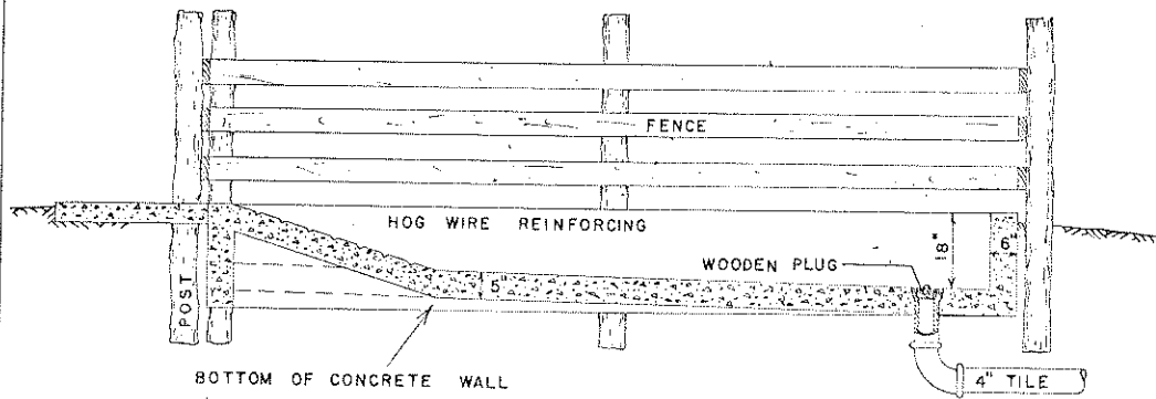
SECTION LENGTHWISE 0 1 2 3 FT.
