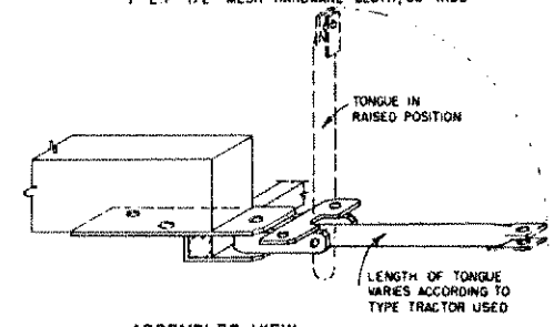
ASSEMBLED VIEW OF HITCH
