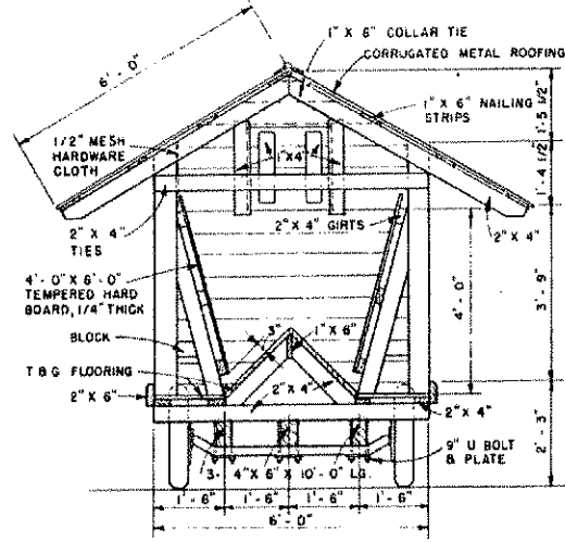
CROSS SECTION SCALE: 0 1 2 3 FT.
