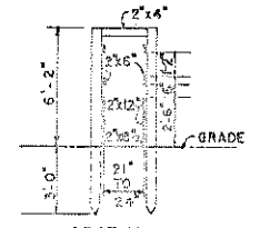
SECTION THRU CHUTE
