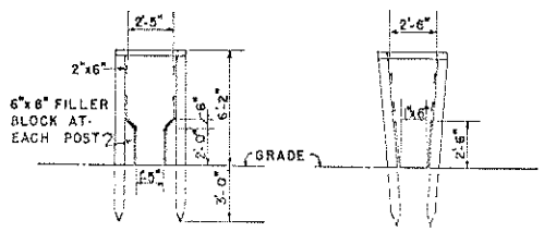
SECTIONS THRU ALTERNATE CHUTES
