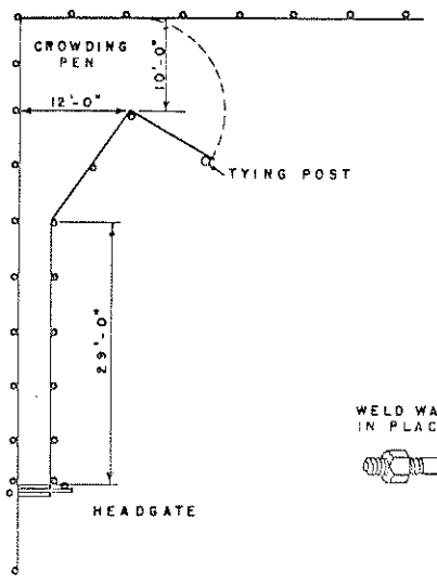
PLAN OF CHUTE IN CORNER OF PASTURE
