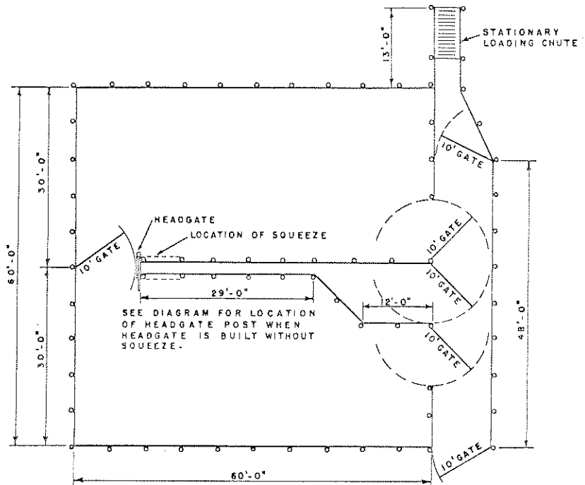
PLAN NO. 1 WITH INTERIOR WORKING CHUTE
