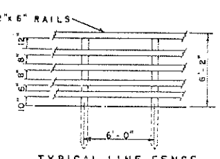
TYPICAL LINE FENCE
