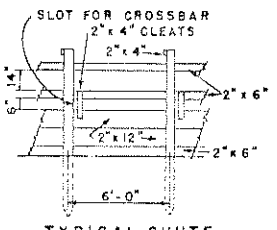
TYPICAL CHUTE
