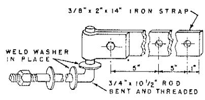
TYPICAL GATE HINGE
