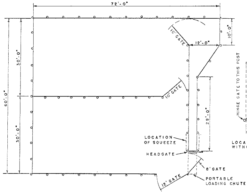
PLAN NO. 2 WITH OUTSIDE WORKING CHUTE
