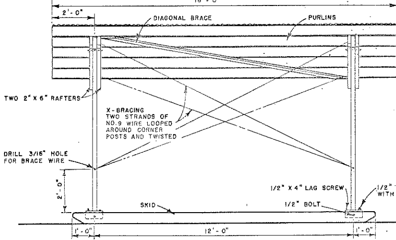
SIDE ELEVATION
