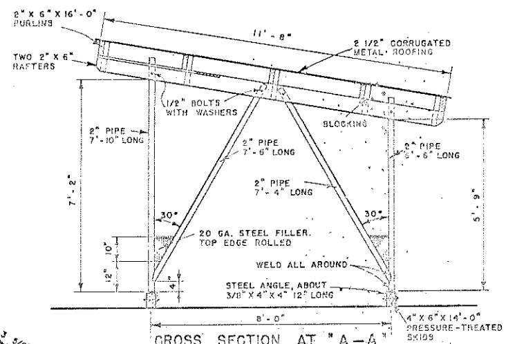
CROSS SECTION AT "A-A" FOR PORTABLE SHADE
