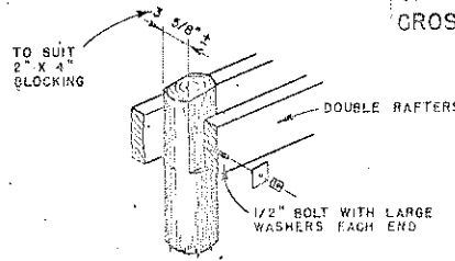
RAFTER CONNECTION DETAIL FOR PERMANENT SHADE
