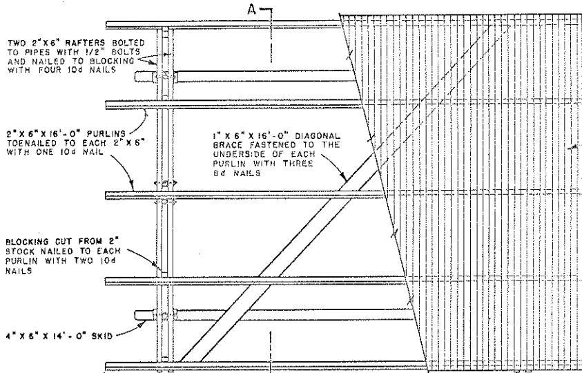
PLAN SHOWING ROOF FRAMING
