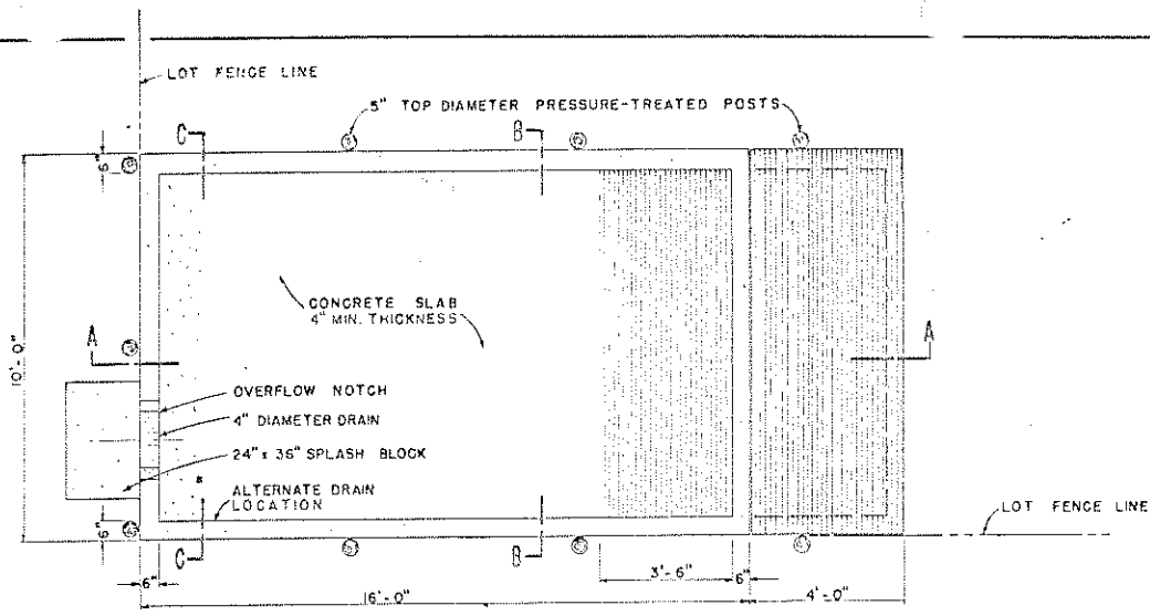
PLAN 0 1 2 3 4 FT.
