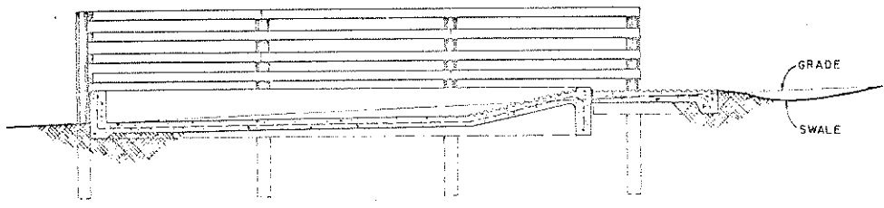
SECTION A-A (SLOPING SITE, PREFERRED)
