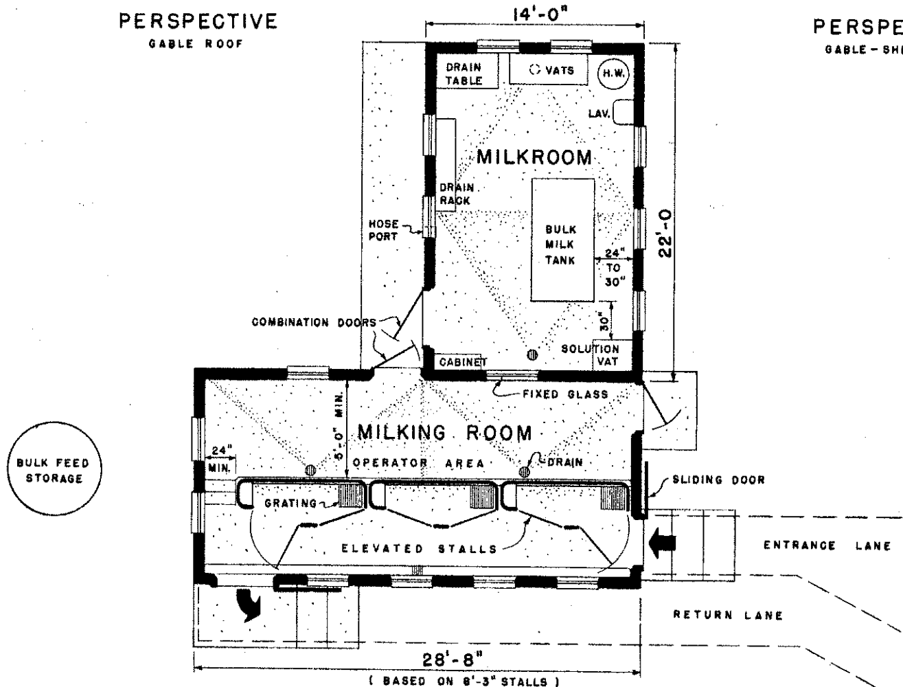
FLOOR PLAN
