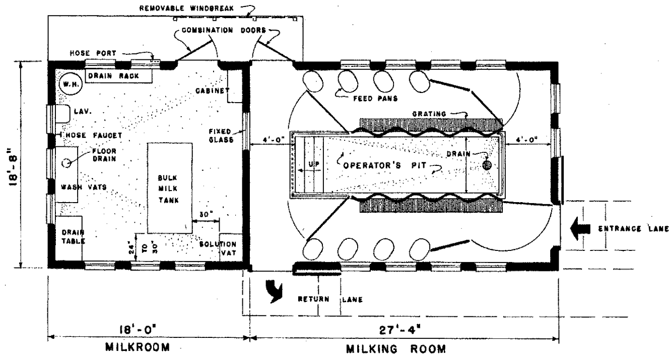
FLOOR PLAN
