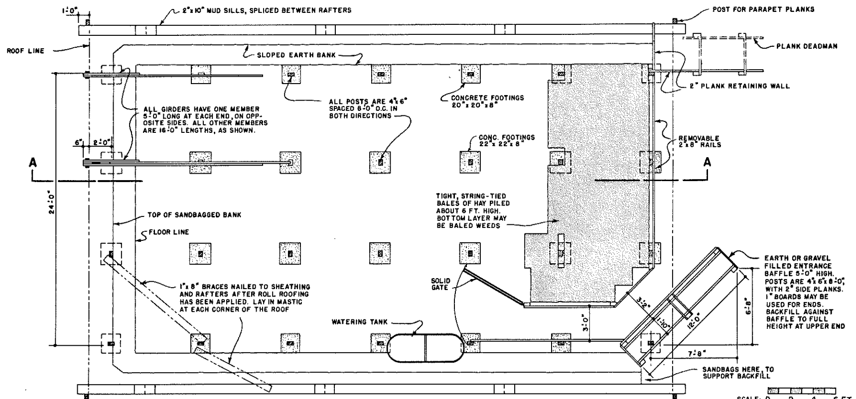
3-BAY PLAN
