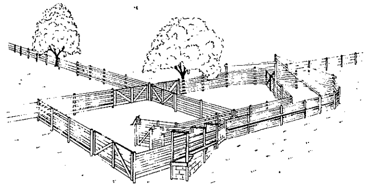
PERSPECTIVE SKETCH
