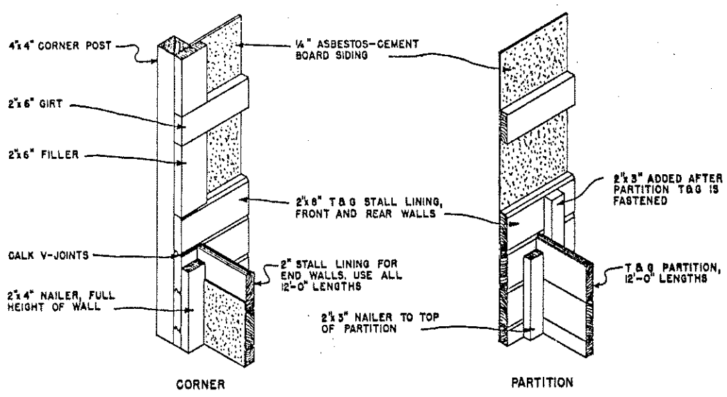
TYPICAL DETAILS
