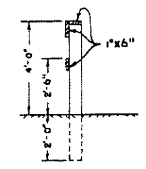
ALTERNATE SECTION
