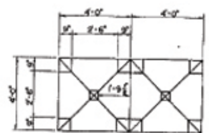
GUSSET CUTTING DETAIL 0 1 2 3 4 FT.
