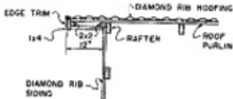
GABLE END DETAIL 0 1 2 FT.
