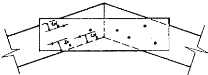
DETAIL A 2x12x4'-0" TIES
