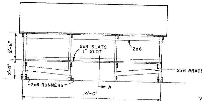
REAR FRAMING
