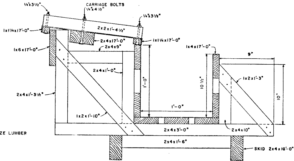
CROSS SECTION
