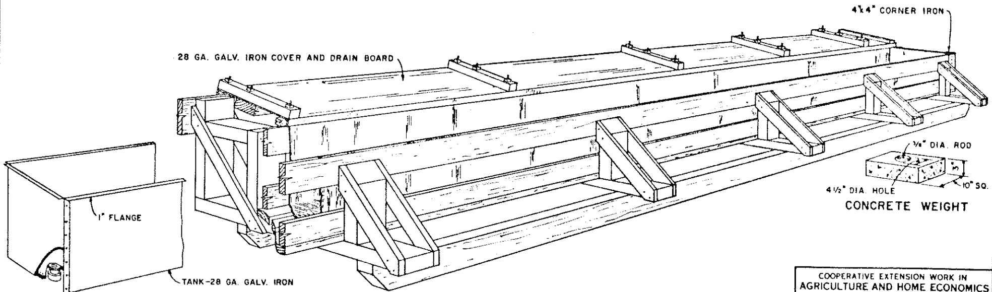
CUTAWAY PERSPECTIVE
