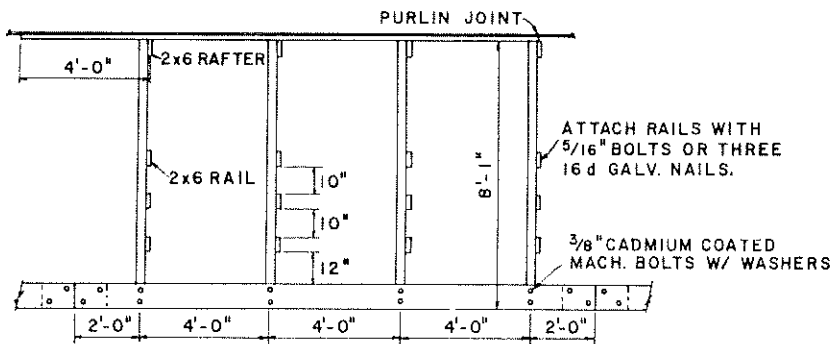
FOUR STALL INTERMEDIATE UNIT (USING 4x4 POSTS)
