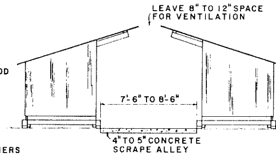
SUGGESTED KENNEL ARRANGEMENT
