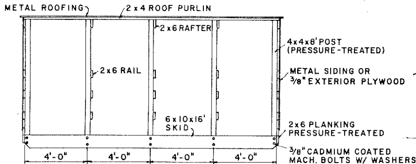
SINGLE FOUR STALL UNIT
