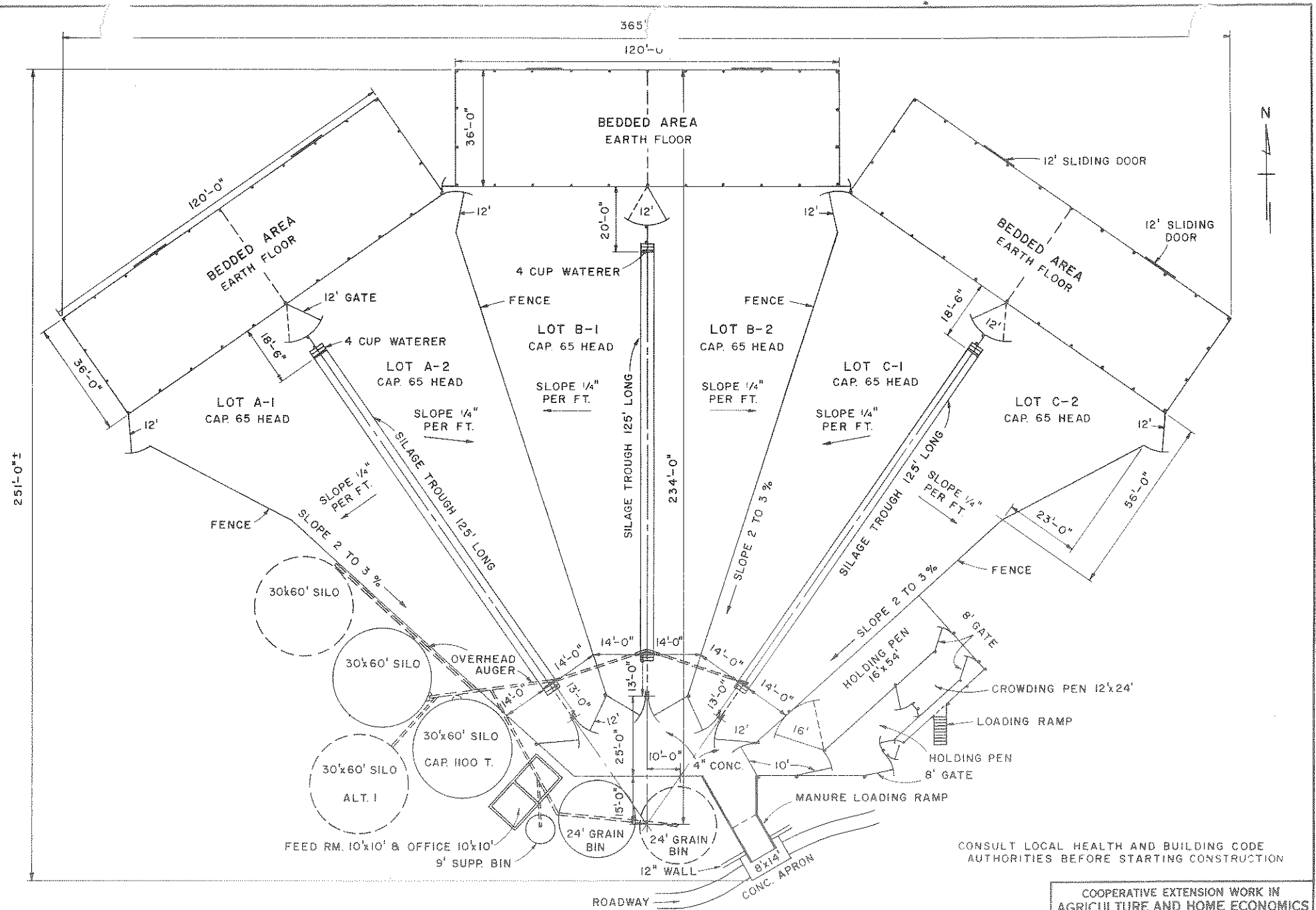
PLAN OF FEED LOTS SCALE: 1"=20' 10' 5' 0 10' 20' 30'
