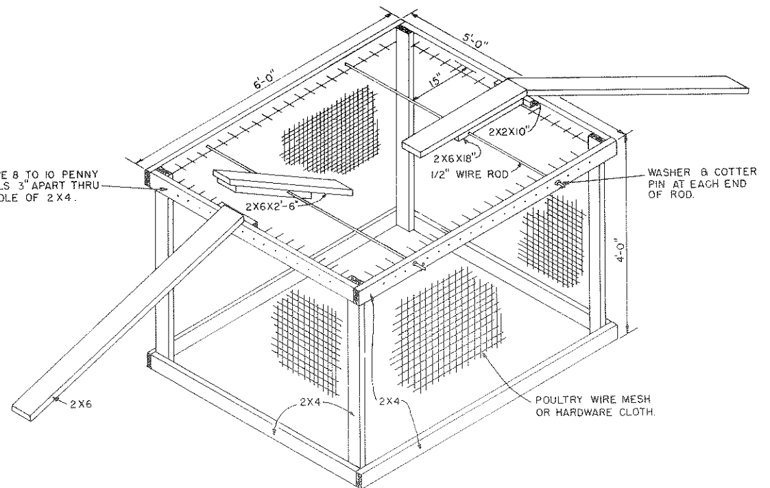
TURTLE BOX TRAP
