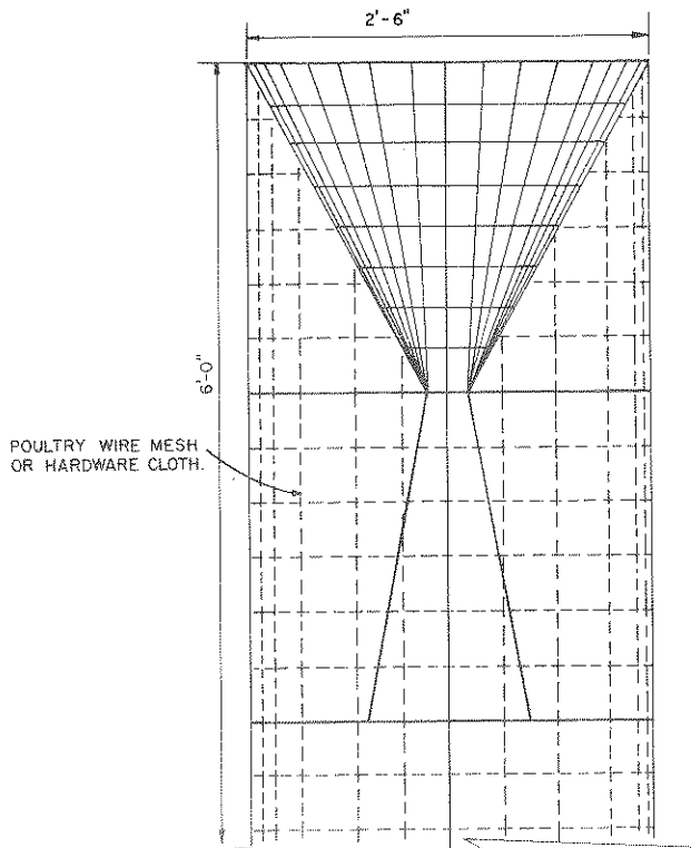
NARROW-MOUTHED FUNNEL TRAP
