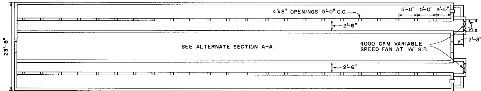
UNDER SLAT VENTILATION LAYOUT
