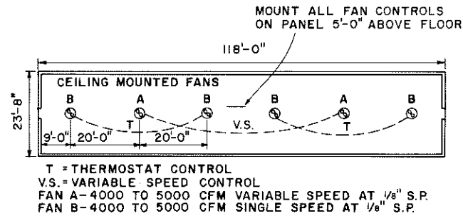
VENTILATION LAYOUT
