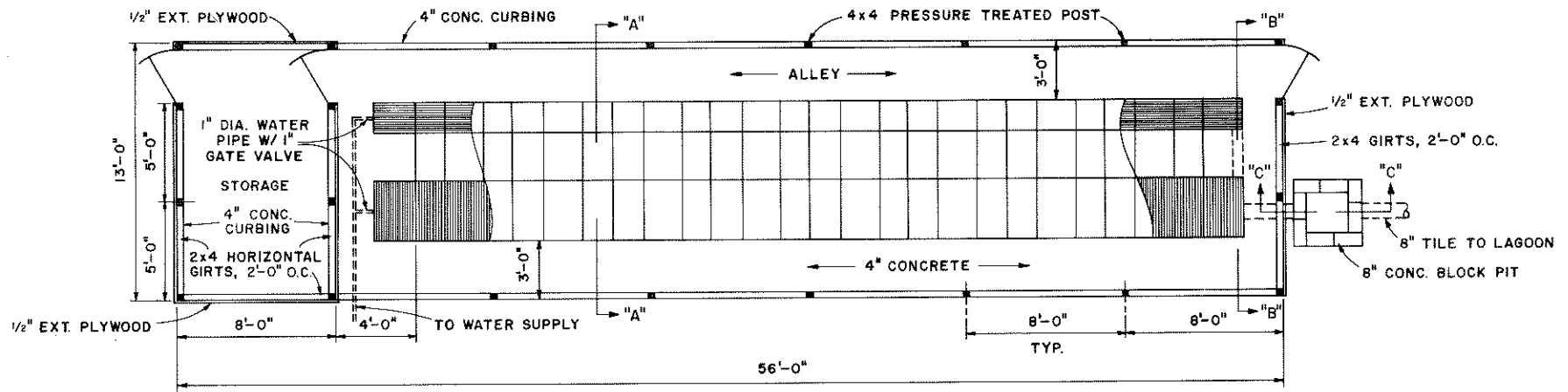
FLOOR PLAN
