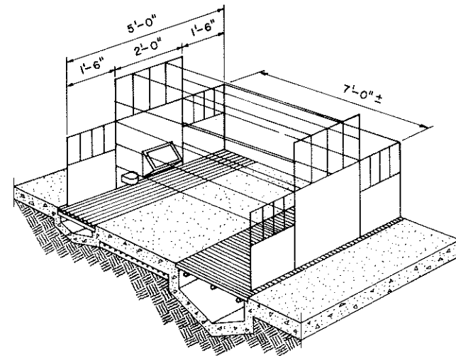
PERSPECTIVE TYPICAL PEN
