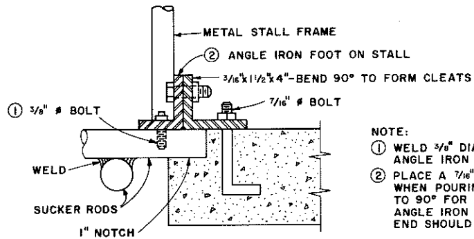
DETAIL FOR ANCHORING STALLS SCALE: NONE
