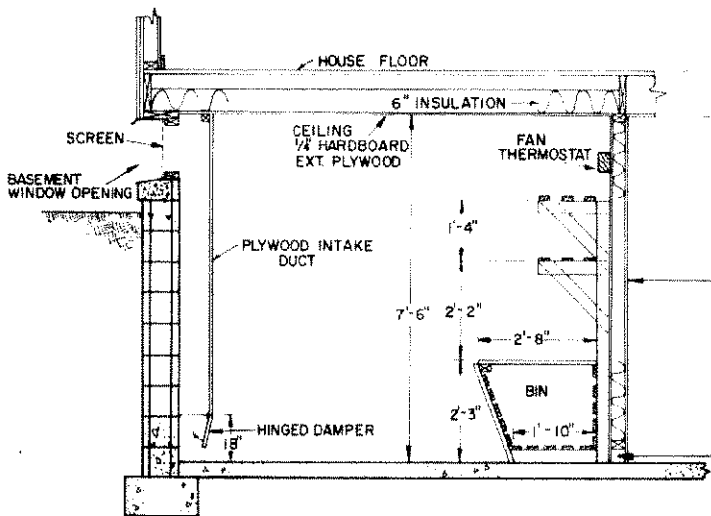
CROSS SECTION
