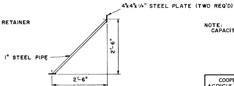
PIPE BRACE
