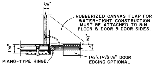
HINGE DETAIL
