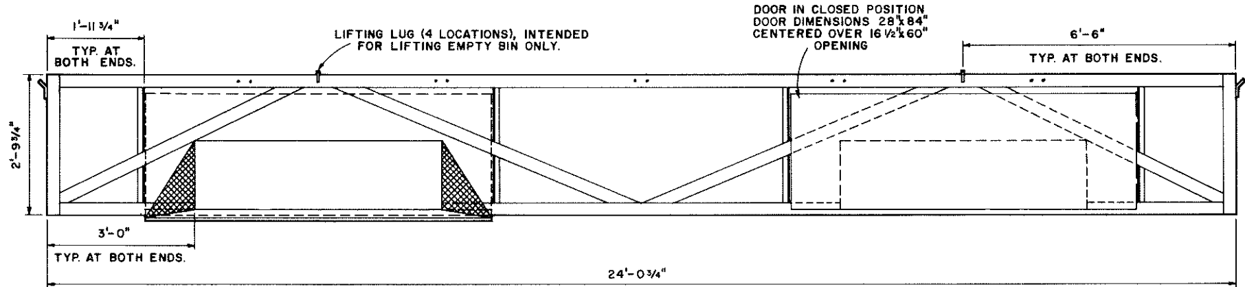
SIDE ELEVATION
