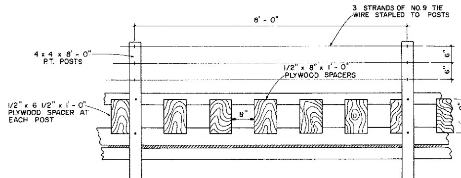
FRONT VIEW SCALE: 3/4" = 1'-0"
