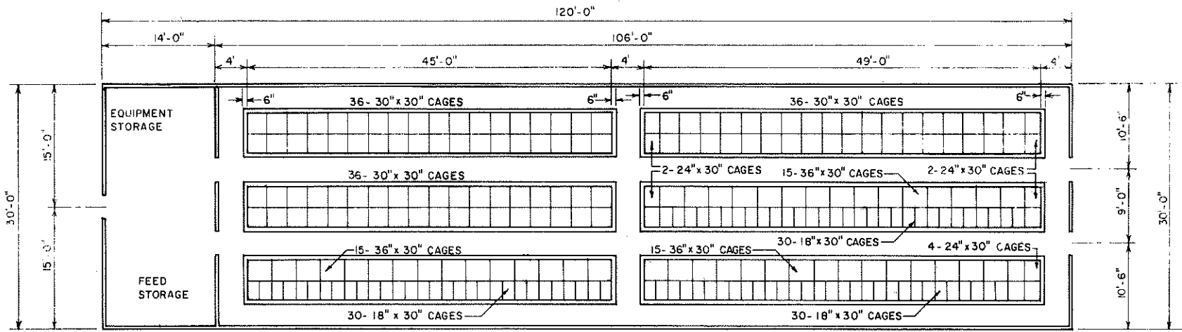
FLOOR PLAN
