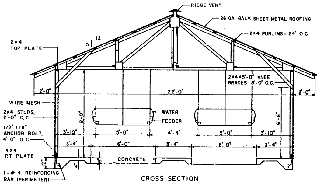
CROSS SECTION
