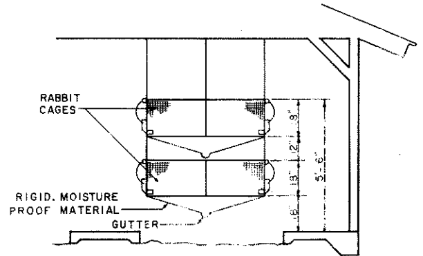
DOUBLE DECKED CAGES
