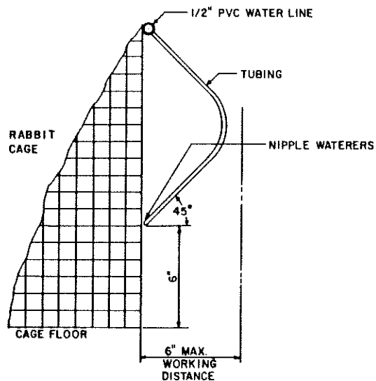
WATER LINE TO CAGES - DETAILS
