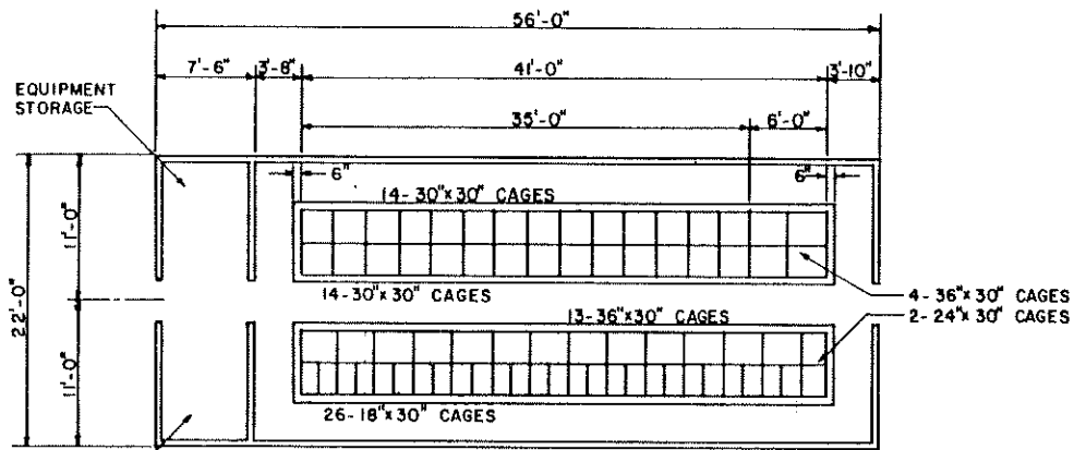
FLOOR PLAN
