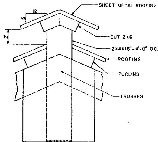
ROOF VENT DETAILS
