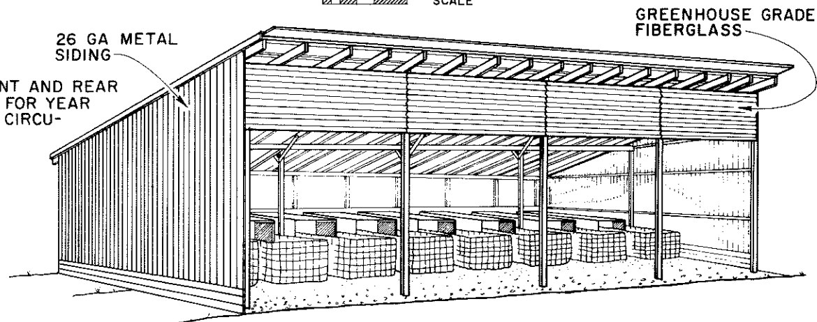
PERSPECTIVE (SIZED FOR 60 COW HERD)
