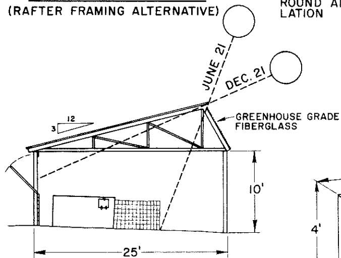
SOLAR PENETRATION (TRUSS FRAMING ALTERNATIVE)
