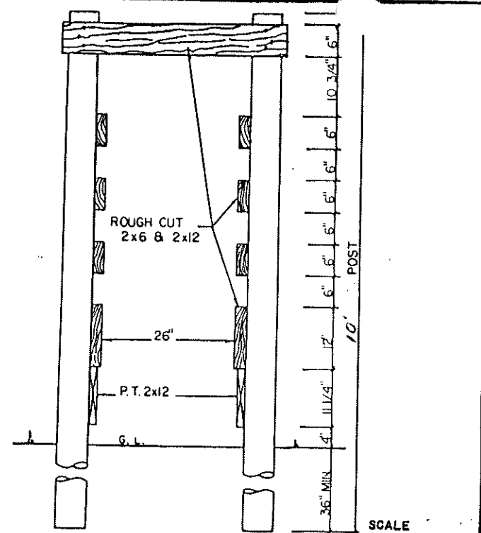
CHUTE SECTION
