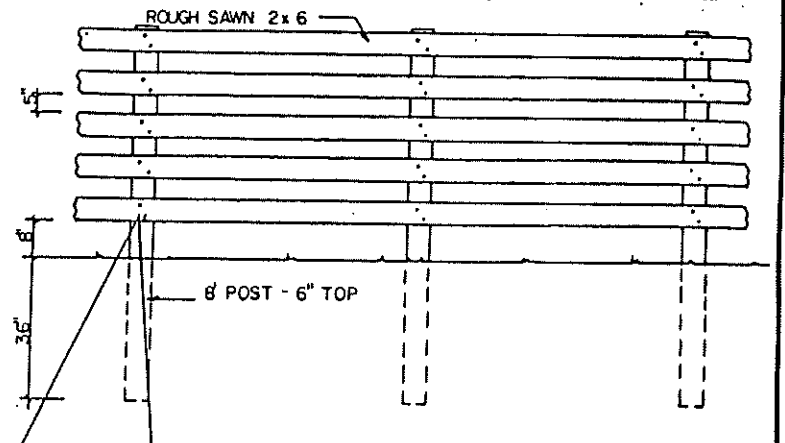
TYPICAL FENCE
