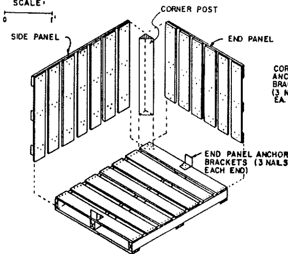
ASSEMBLY DIAGRAM
