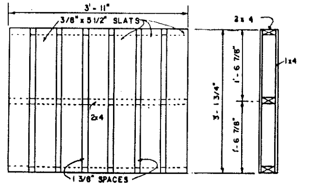
TOP VIEW END VIEW
