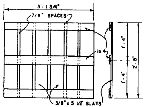
FRONT VIEW EDGE VIEW END PANEL SCALE: 0 1' (2 REQ'D)
