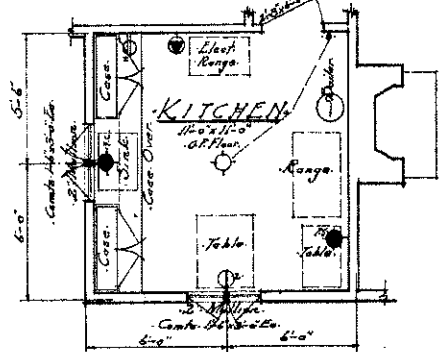
ALTERNATE KITCHEN PLAN Scale 1/4" = 1'-0"
