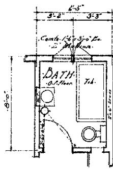
ALTERNATE BATH PLAN Scale 1/4" = 1'-0"
