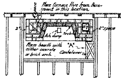
FRAMING FOR FIREPLACE
