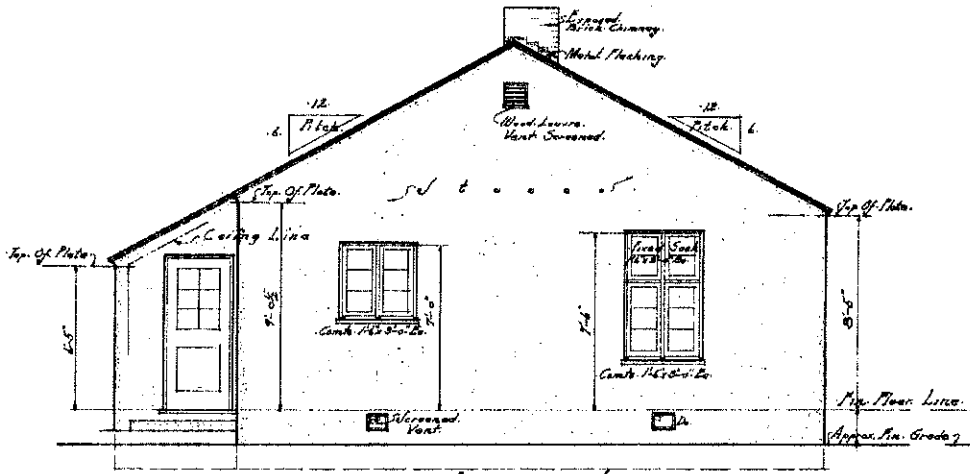
SIDE ELEVATION Scale 1/4" = 1'-0"
