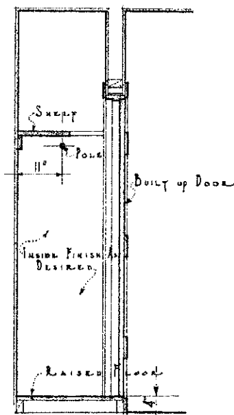
SECTION X-X
