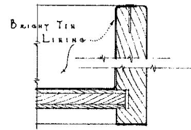
• FULL-SIZE-DETAIL • OF METAL-LINED DRAWER •
