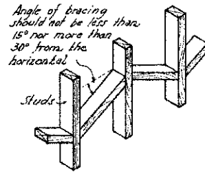
BRACING BETWEEN STUDS
