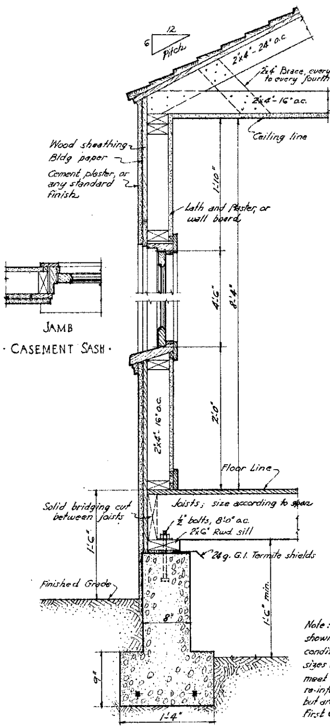
• WITH SPREAD FOOTING
