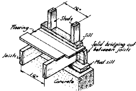
CONSTRUCTION AT SILL
