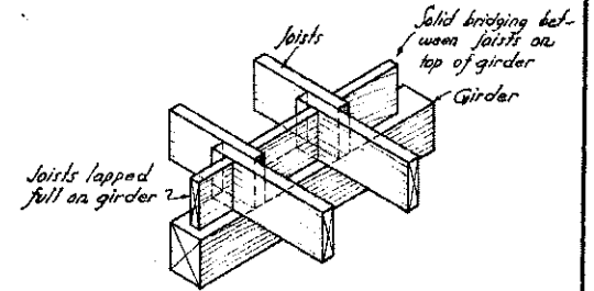
JOISTS LAPPED ON TOP OF GIRDER
