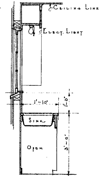
SECTION C-C
