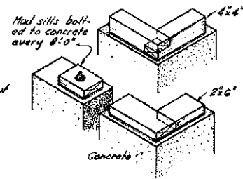
MUD SILLS AT CORNER
