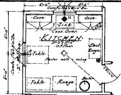
ALTERNATE KITCHEN PLAN Scale 1/4" = 1'-0"
