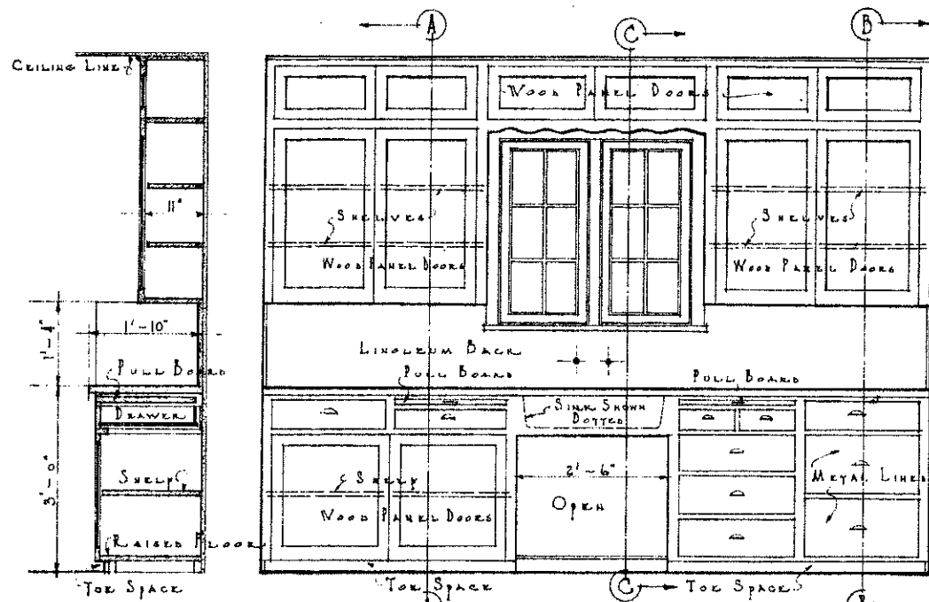
SECTION A-A • ELEVATION OF KITCHEN SHOWING CASES •
