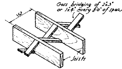
CROSS BRIDGING BET. JOISTS
