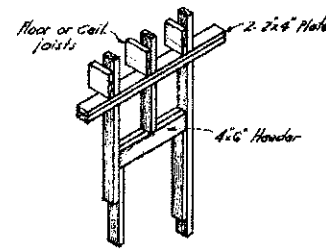
FRAMING FOR OPENINGS UNDER 3'-0" WIDE
