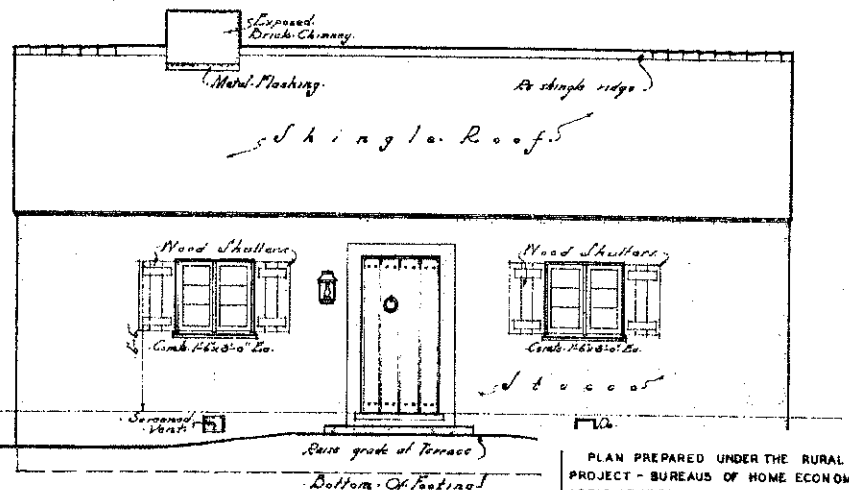
FRONT ELEVATION Scale: 1/4" = 1'-0"
