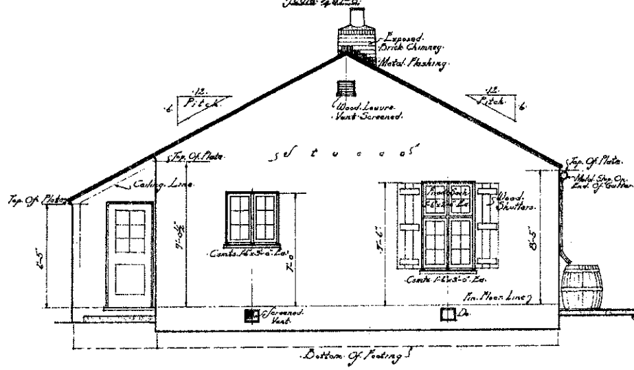
SIDE ELEVATION Scale 1/4" = 1'-0"
