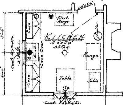
ALTERNATE KITCHEN PLAN Scale 1/4" = 1'-0"
