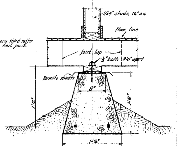
INTERIOR WALL UNDER BEARING PARTN.
