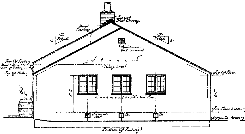
SIDE ELEVATION Scale 1/4" = 1'-0"
