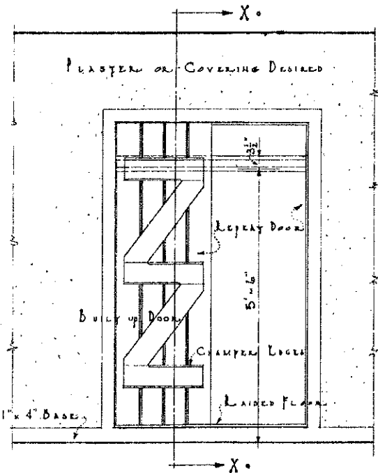
SECTION X-X • ELEVATION OF TYPICAL WARDROBE •
