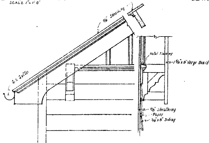
DETAIL OF GABLE ENDS
