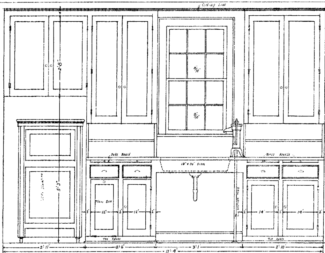
ELEVATION DETAIL 'A' FOR CABINETS
