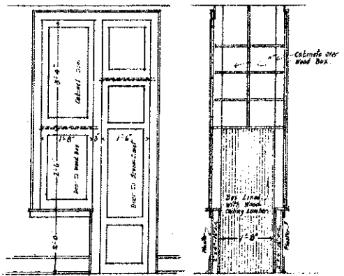
DETAIL 'B' FOR WOOD BOX & BROOM CLOSET
