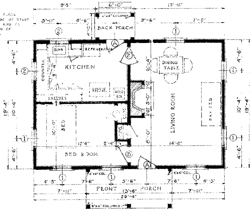
FLOOR PLAN SCALE 3/4\"/>
