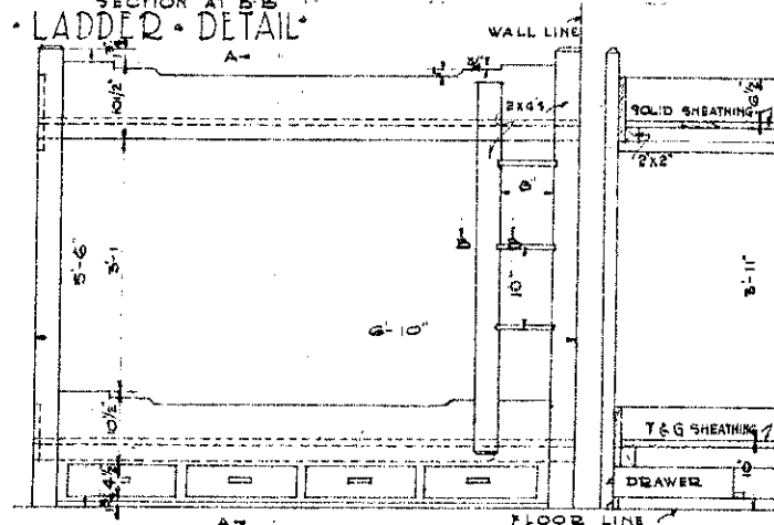
ELEVATION OF DOUBLE DECK BUNK SCALE 3/4" = 1'-0"
