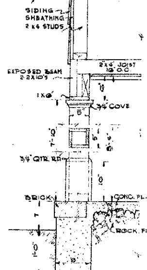
SECTION AA PORCH DETAIL SCALE 1" = 1'-0"
