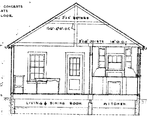
SECTION SCALE 1/4" = 1'-0"
