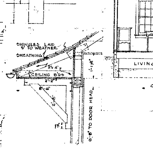
DETAIL OF SHELTER OVER REAR ENTRANCE SCALE 3/4" = 1'-0"
