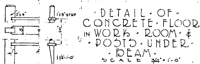
DETAIL OF CONCRETE FLOOR IN WORK ROOM & POSTS UNDER BEAM SCALE 3/4" = 1'-0"
