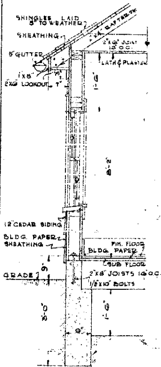
SECTION THRU WALL SCALE 3/4" = 1'-0"
