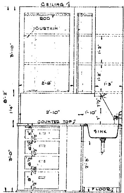
KITCHEN CABINET DETAIL SCALE 1/4" = 1'-0"
