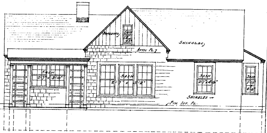
SOUTHEAST ELEVATION
