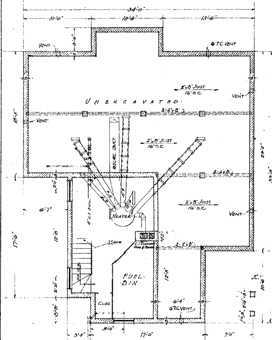
BASEMENT PLAN
