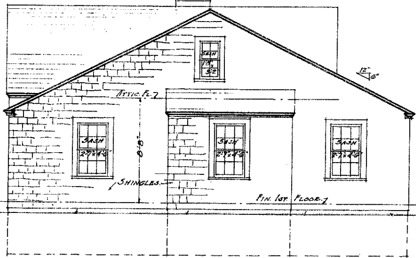
NORTHEAST ELEVATION
