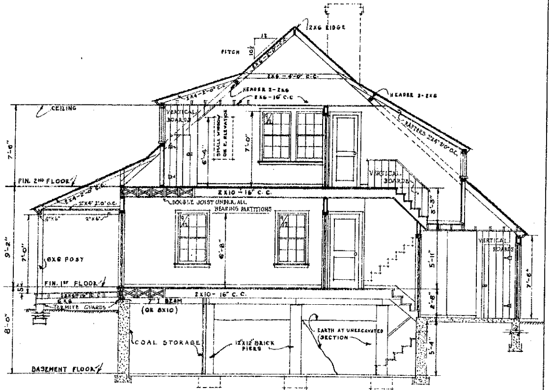
SECTION ON LINE "XX" SCALE 1/4" = 1'-0"
