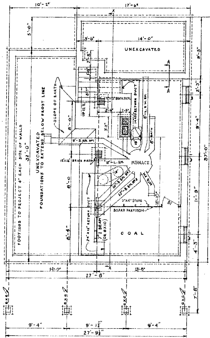
BASEMENT PLAN SCALE 1/4" = 1'-0"
