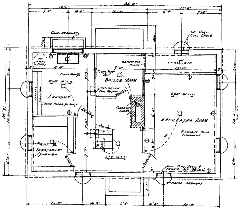
..BASEMENT PLAN.. SCALE 1/4"=1'-0"
