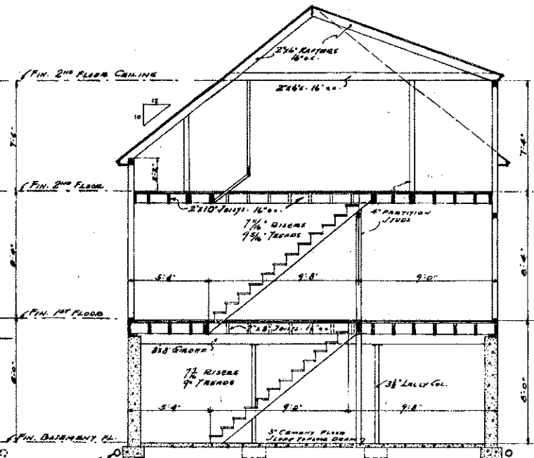
..CROSS SECTION A-A.. ..INDICATING FRAMING.. SCALE 1/4"=1'-0"
