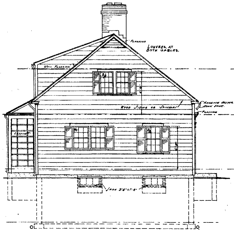
.. LEFT SIDE ELEVATION .. SCALE 1/4"=1'-0"
