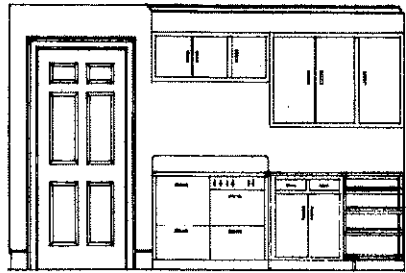
ELEVATIONS - SHOWING KITCHEN CABINETS SCALE 3/4" = 1'-0"
