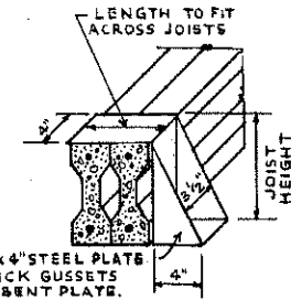
HANGER DETAIL
