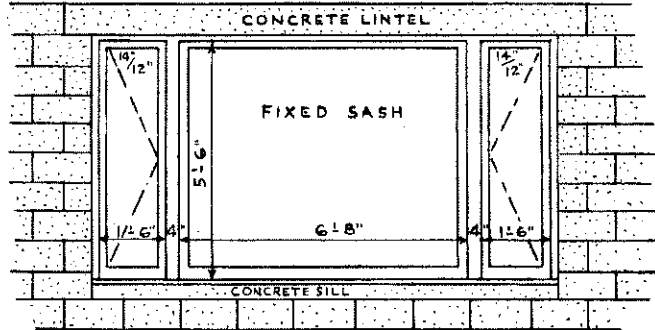
DETAIL OF WINDOW
