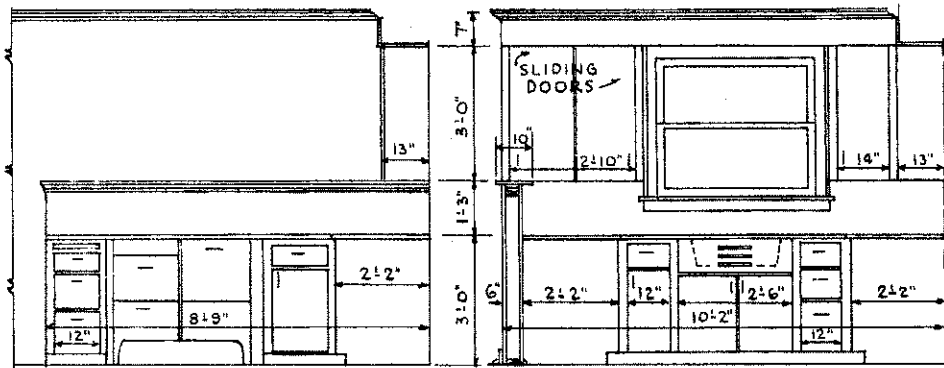
DETAILS OF KITCHEN CABINETS
